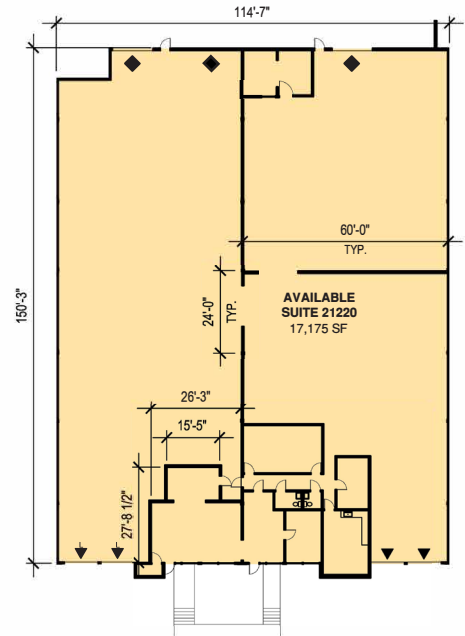
SUITE 21234 1/32" = 1'-0"
