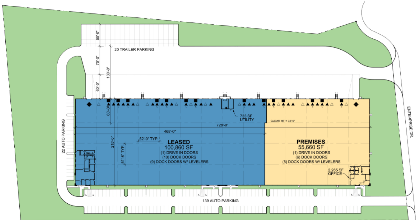
SITE PLAN
