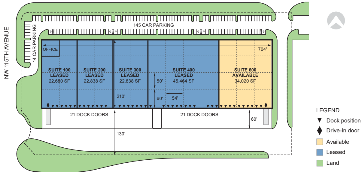
OVERALL AREA PLAN - 34,020 SF
