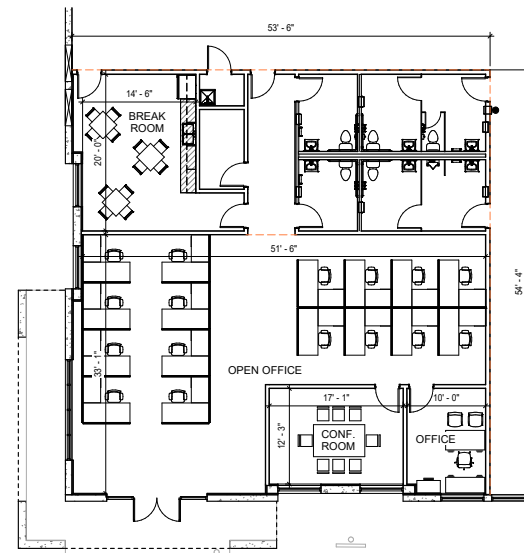
OFFICE SPACE - 2,930 SF
