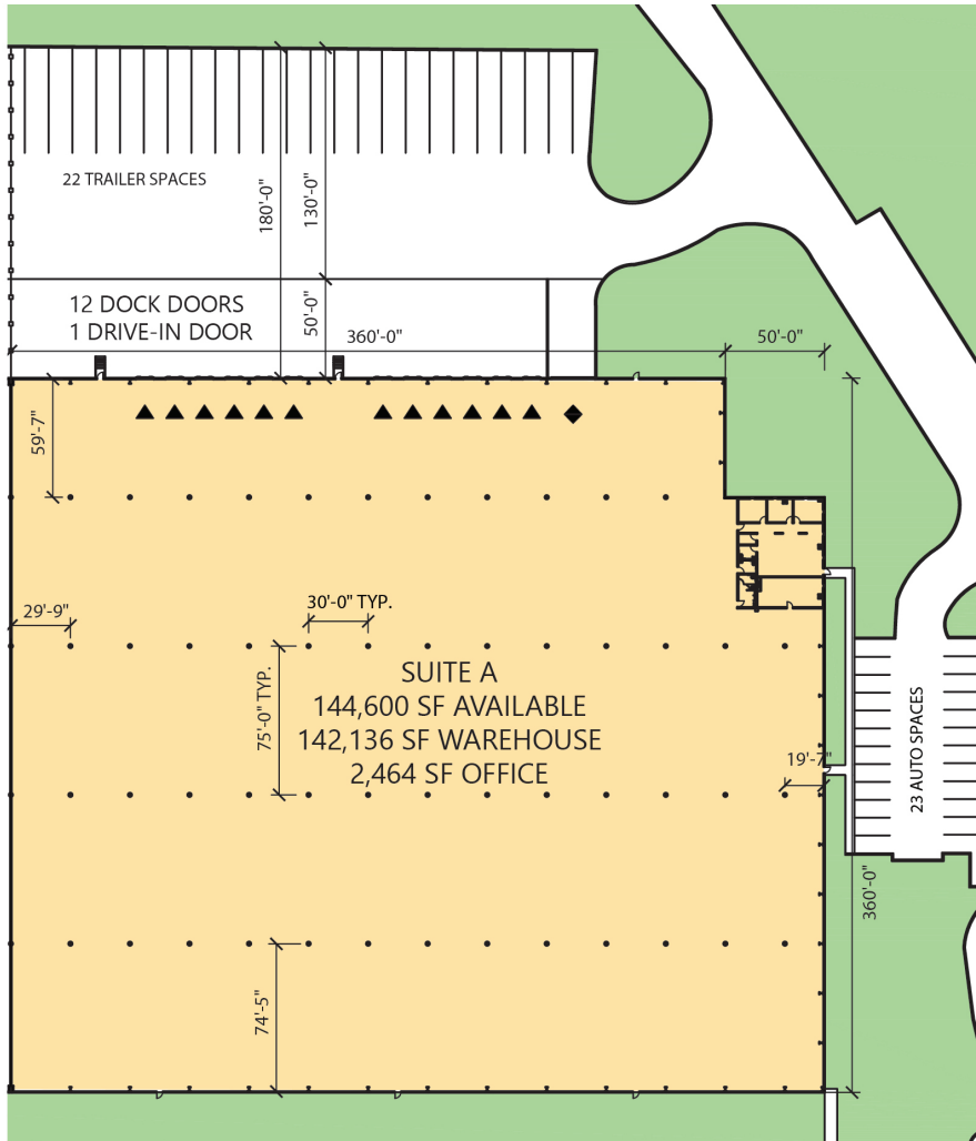
KEY PLAN
