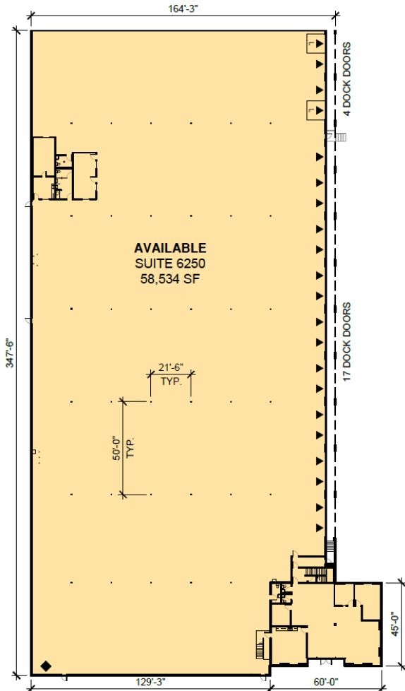
FLOOR & MEZZANINE PLANS NOT TO SCALE
