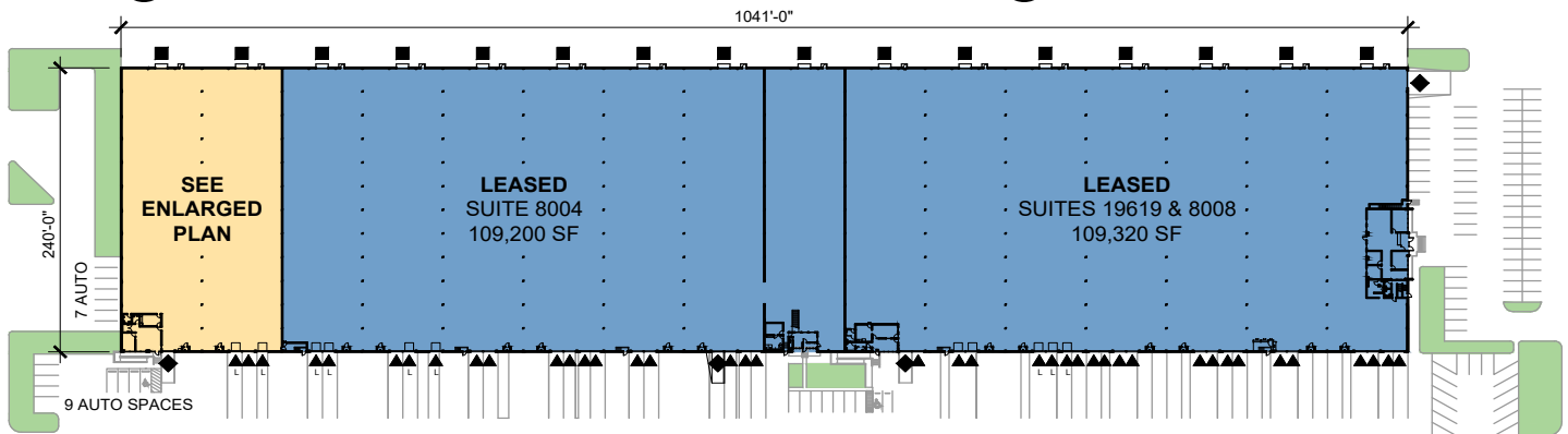
OVERALL SITE PLAN 1" = 100'-0"
