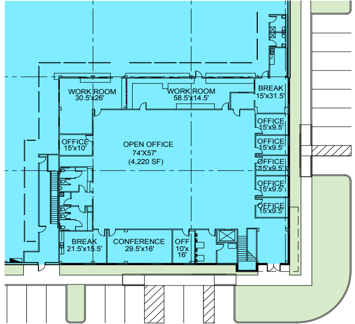
South Office | 10,377 SF
