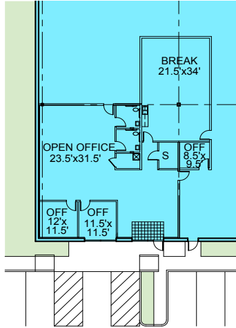
North Office | 2,796 SF
